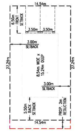
DOUBLE WIDES (15 TOTAL) SCALE: 1:250
