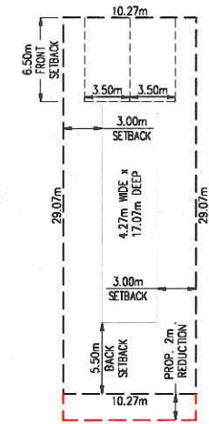
SINGLE WIDES (53 TOTAL) SCALE: 1:250
