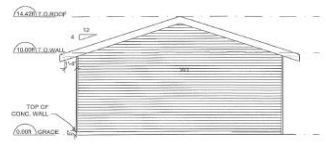
4 West Elevation Scale: 1/4" = 1'-0"
