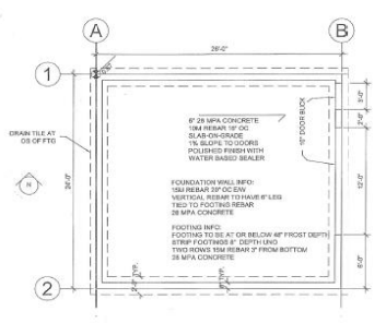
1 Foundation Plan Scale: 1/4" = 1'-0"
