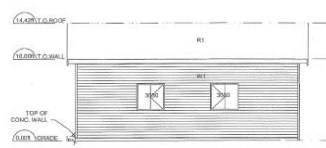
6 North Elevation Scale: 1/4" = 1'-0"
